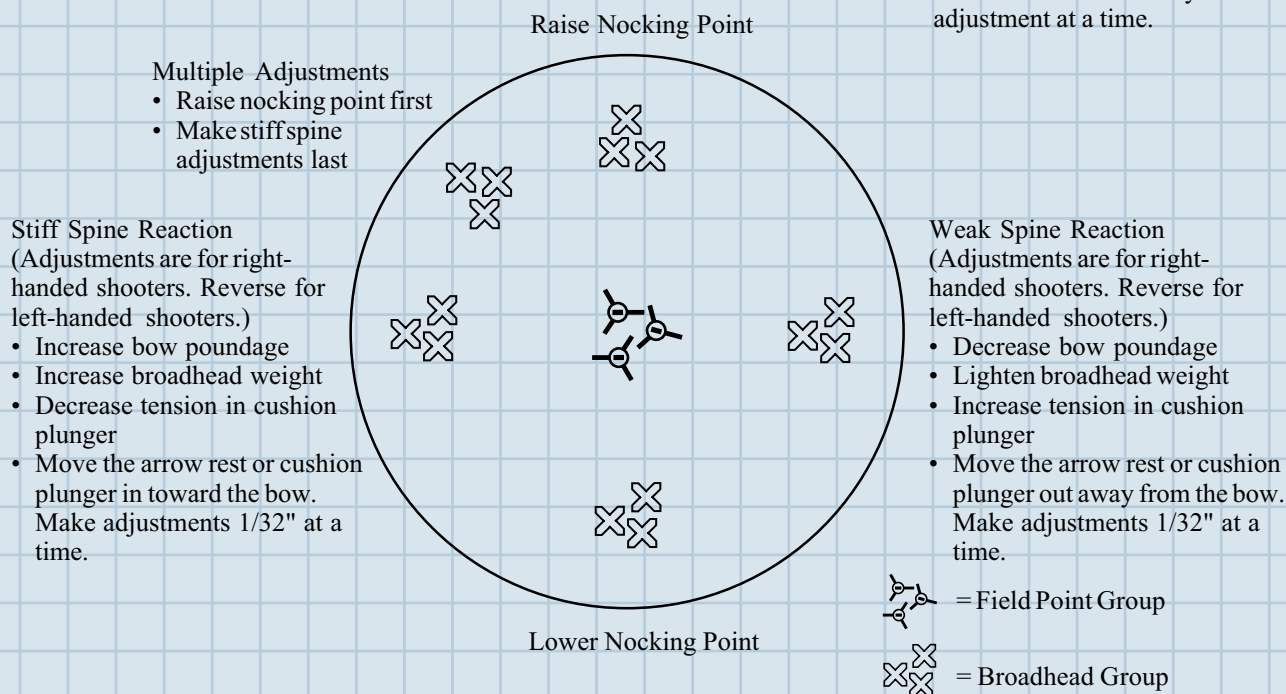
Fig. 20 Broadhead Tuning
